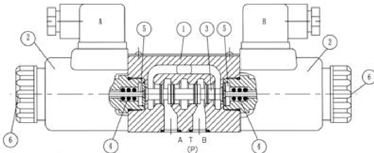
Type WE6...61B/
