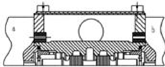
Type WE10...20B/OA
