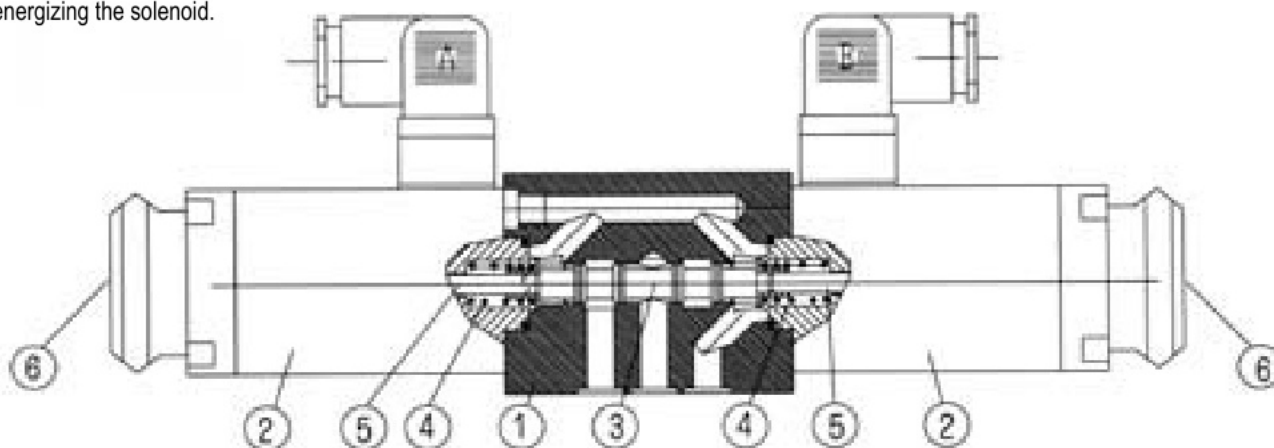
Type WE5
