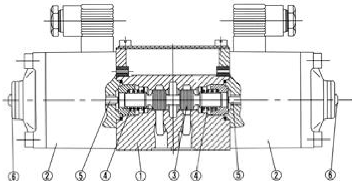
Type WE10...20B/A...
